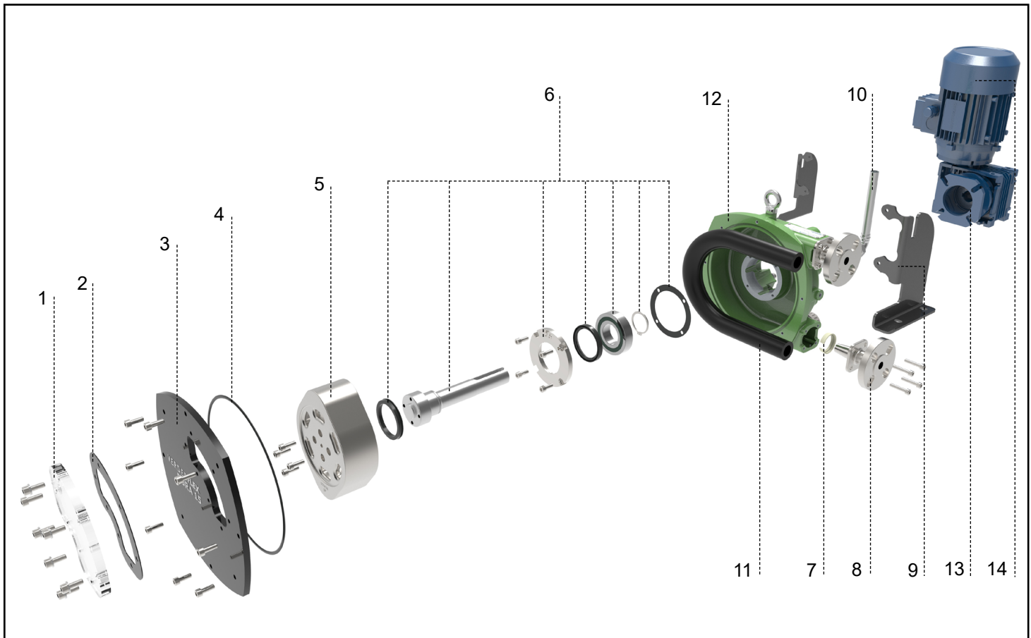
Figure 1 Layout - Dura MK III 15, 25, 35 Generic View
